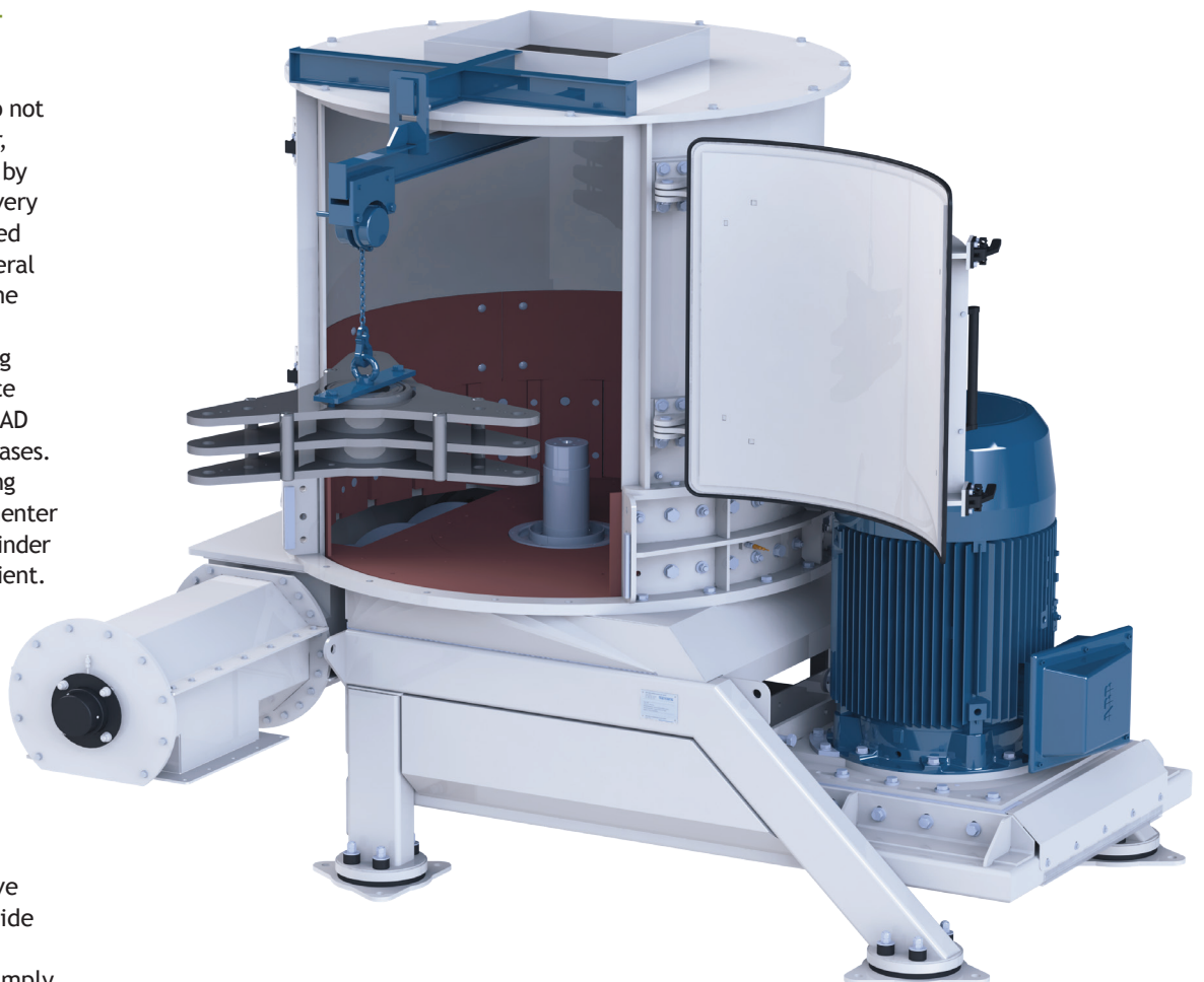
Maintenance friendly wide opening door, option: crane traverse for easy change of the rotor and stairs in front of the door
